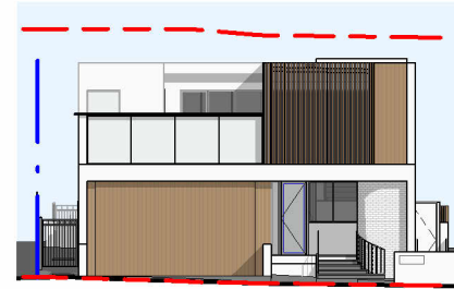
2 SOUTH ELEVATION 1 : 300
